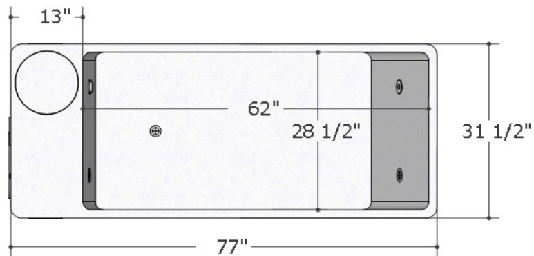
Top Section
